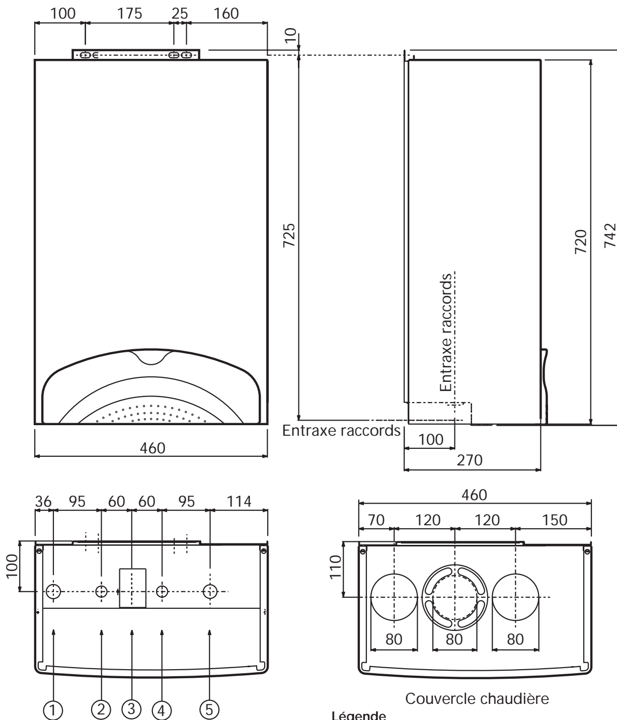
Raccords chaudière
